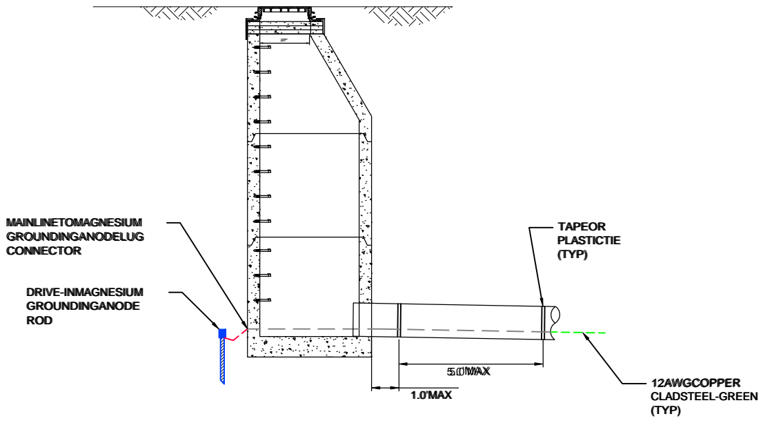
SEWER MANHOLE-SECTION VIEW NOSCALE
