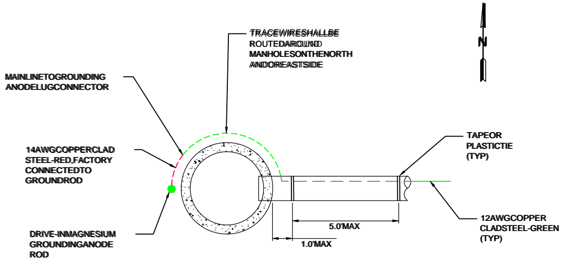
SEWER MANHOLE-PLAN VIEW NOSCALE
