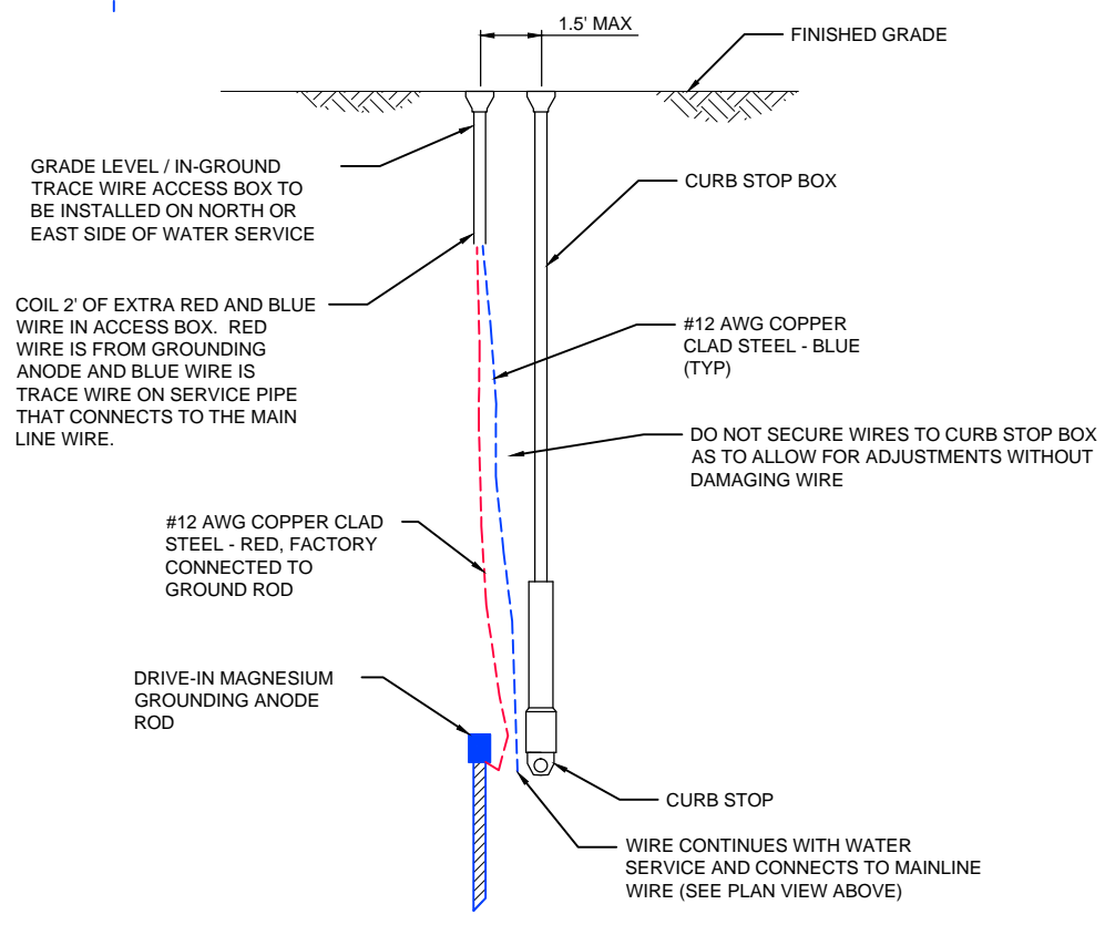
WATER SERVICE - SECTION VIEW NO SCALE
